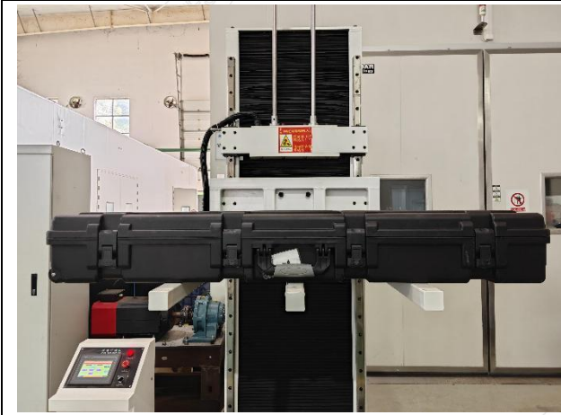
Fig.3-5 Drop test Operation - Surface Schematic Diagram
