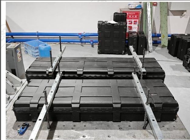
Fig.2-3 Vibration Test Subject Installation Status - X-Axis
